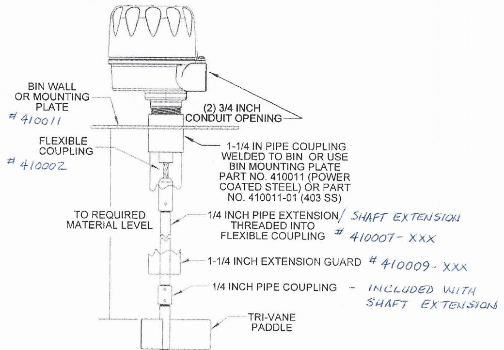
Figure 2: Top Mount Installation
