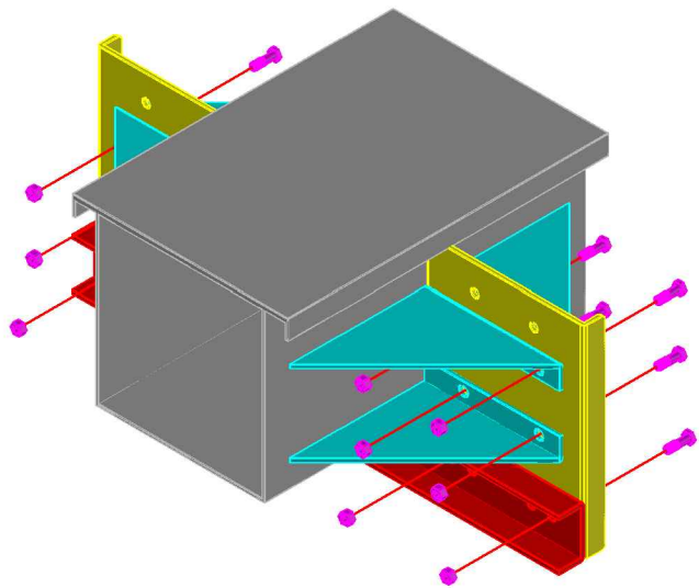
SQUARE END ANCHOR ASSEMBLY
