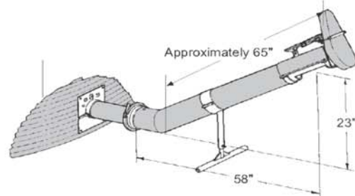
Add 5" to discharge height per each foot of extension.
