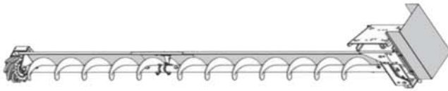
9" O.D. 1/4" Flight on 2 7/8" tube. Drive includes 3 to 1 Oil Bath Reducer. Capacity rated at ~1280 BPH per 100 RPM
