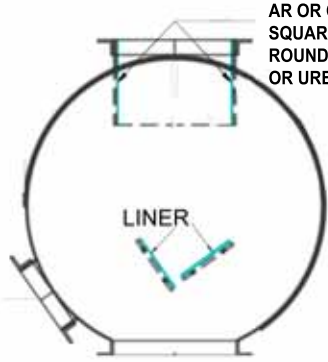
VERTICAL DROP FLOW RETARDER
