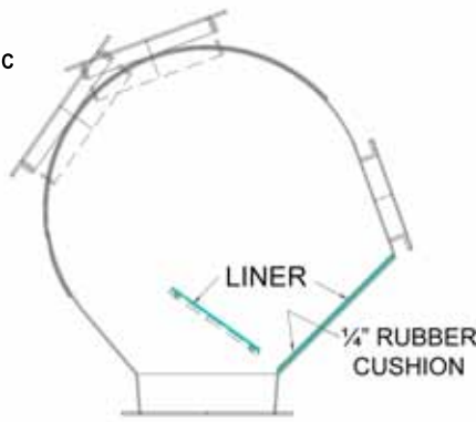
IN-LINE BACKDRAFT DAMPER
